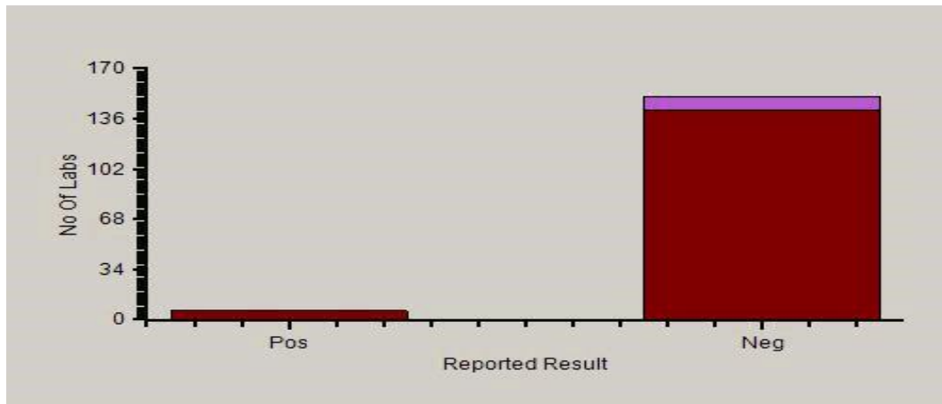
Frequency Histogram
