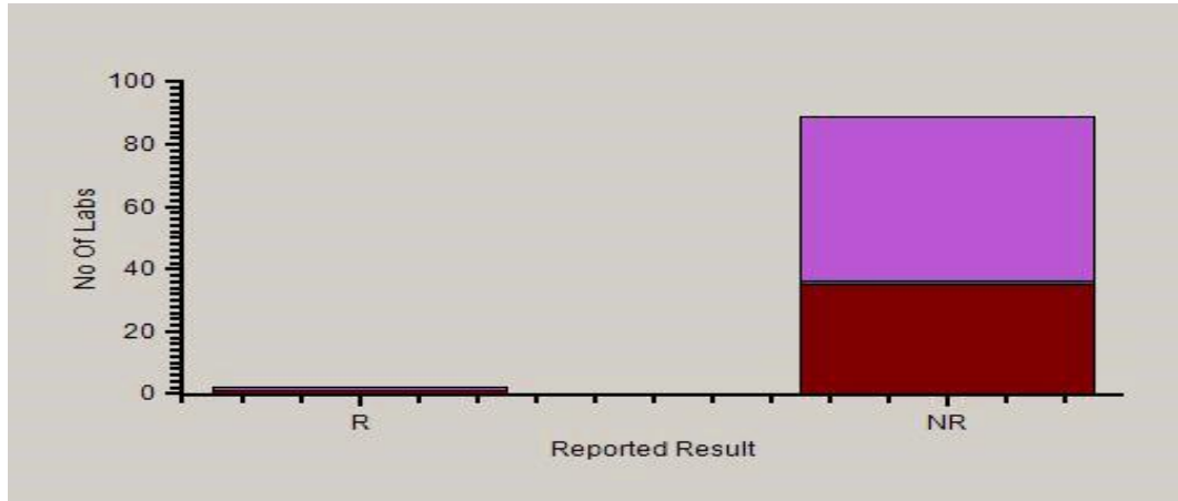
Frequency Histogram
