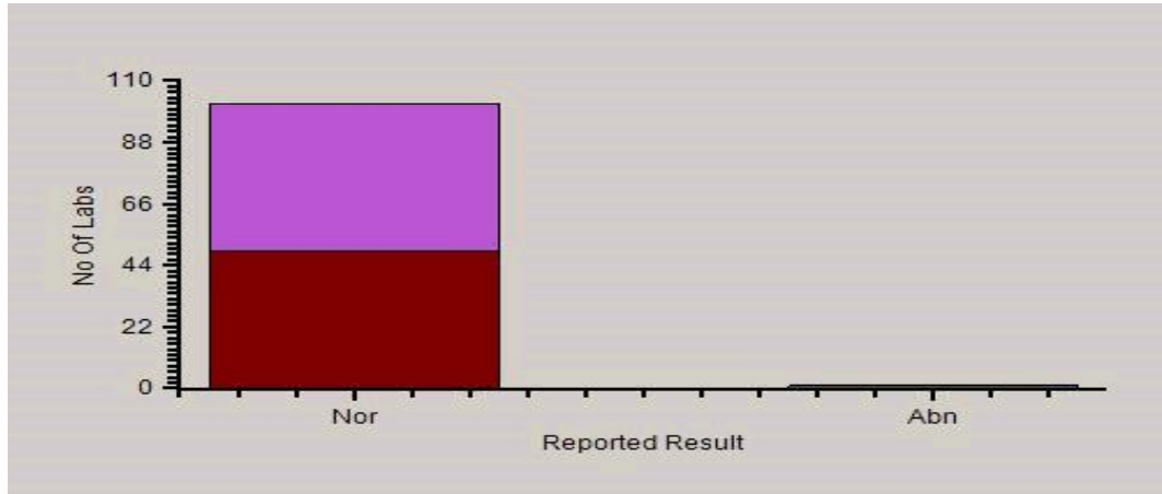
Frequency Histogram
