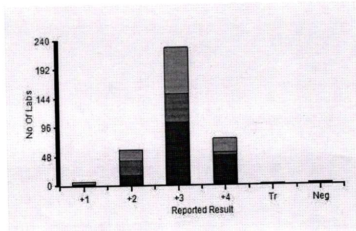
Frequency Histogram
