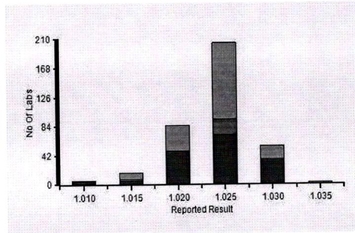
Frequency Histogram
