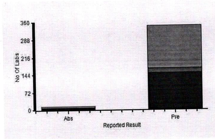
Frequency Histogram
