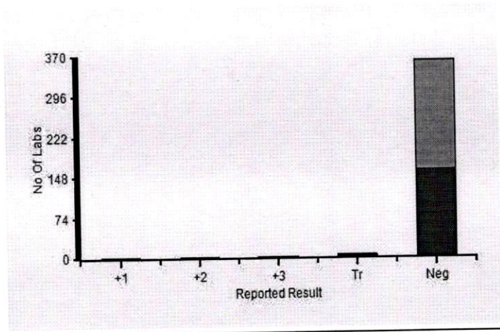
Frequency Histogram
