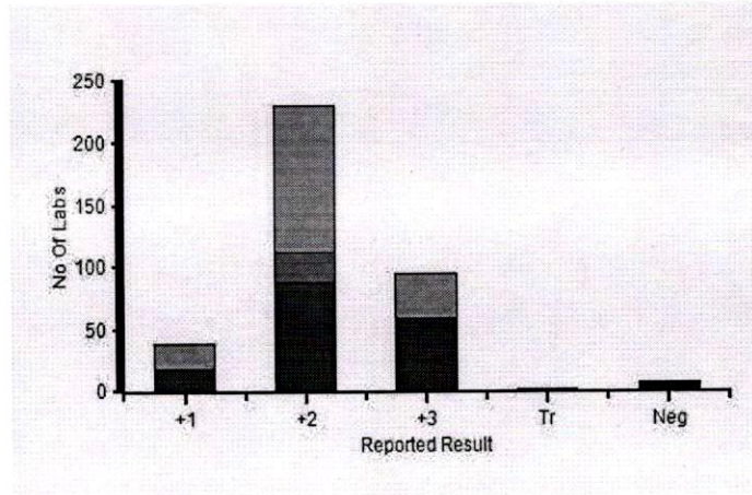
Frequency Histogram
