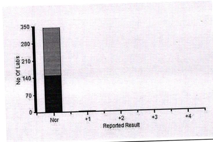
Frequency Histogram
