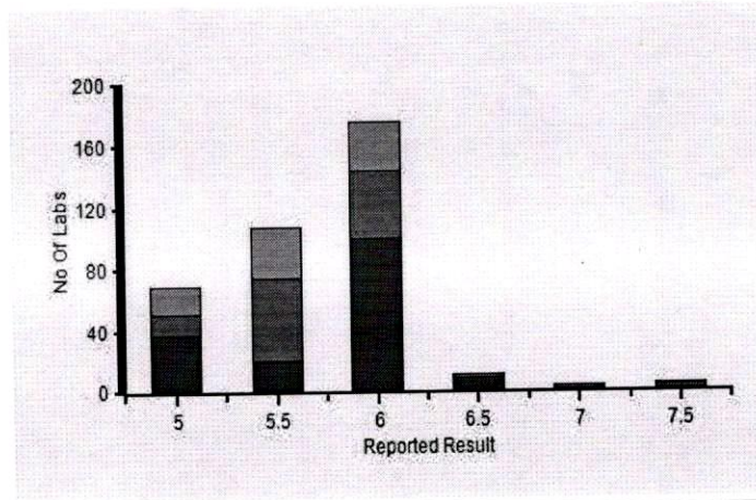
Frequency Histogram
