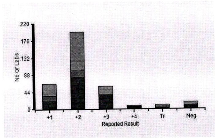
Frequency Histogram
